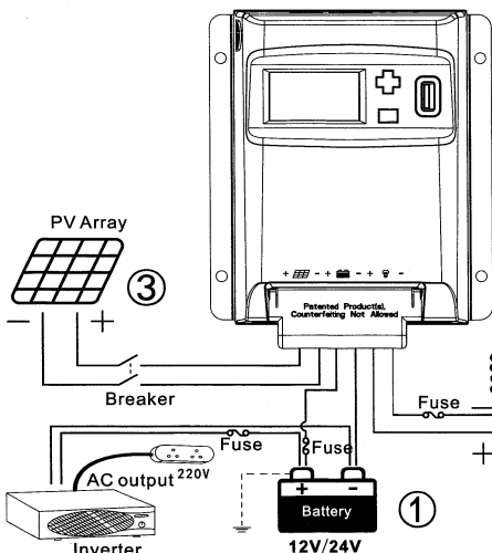
Photo 2 Connection diagram
